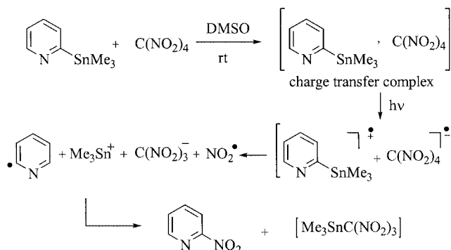
Scheme 3. Nitration of 2-(trimethylstannyl)pyridine by TNM under irradiation
