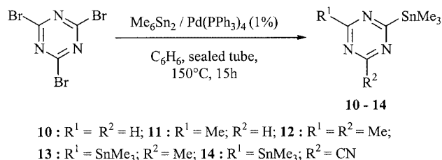
Scheme 2. Reaction between cyanuryl bromide and hexamethylditin
