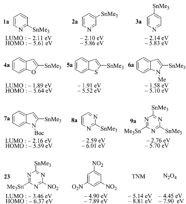
Figure 2. Evaluation of the energies of HOMO and LUMO orbitals
