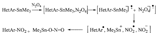
Scheme 4. Nitration of heteroaryltrimethyltins by N 2 O 4
